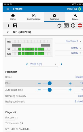
Parameter screen with visualised detection field in the Sensor Settings section.
